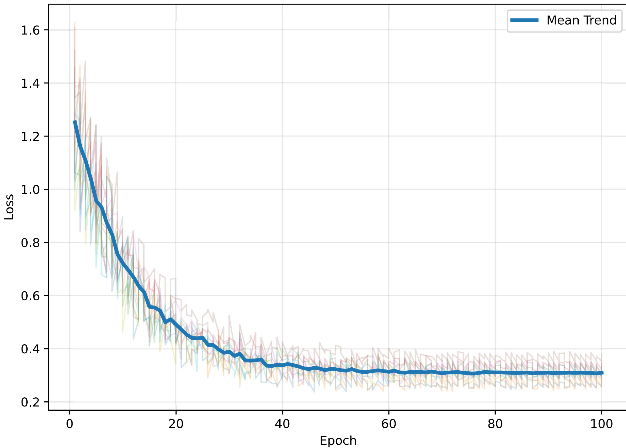
GNN Training Dynamics
