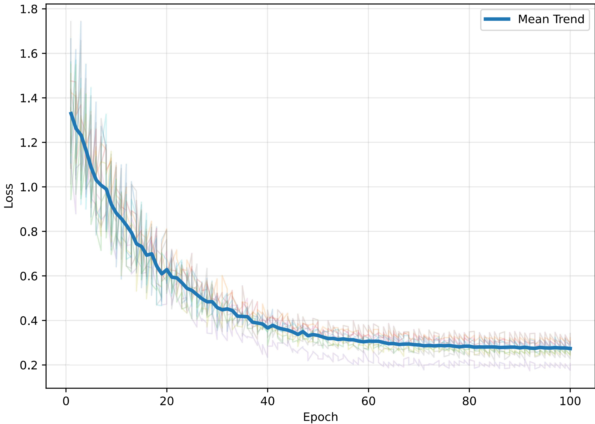
TRANSFORMER Training Dynamics
