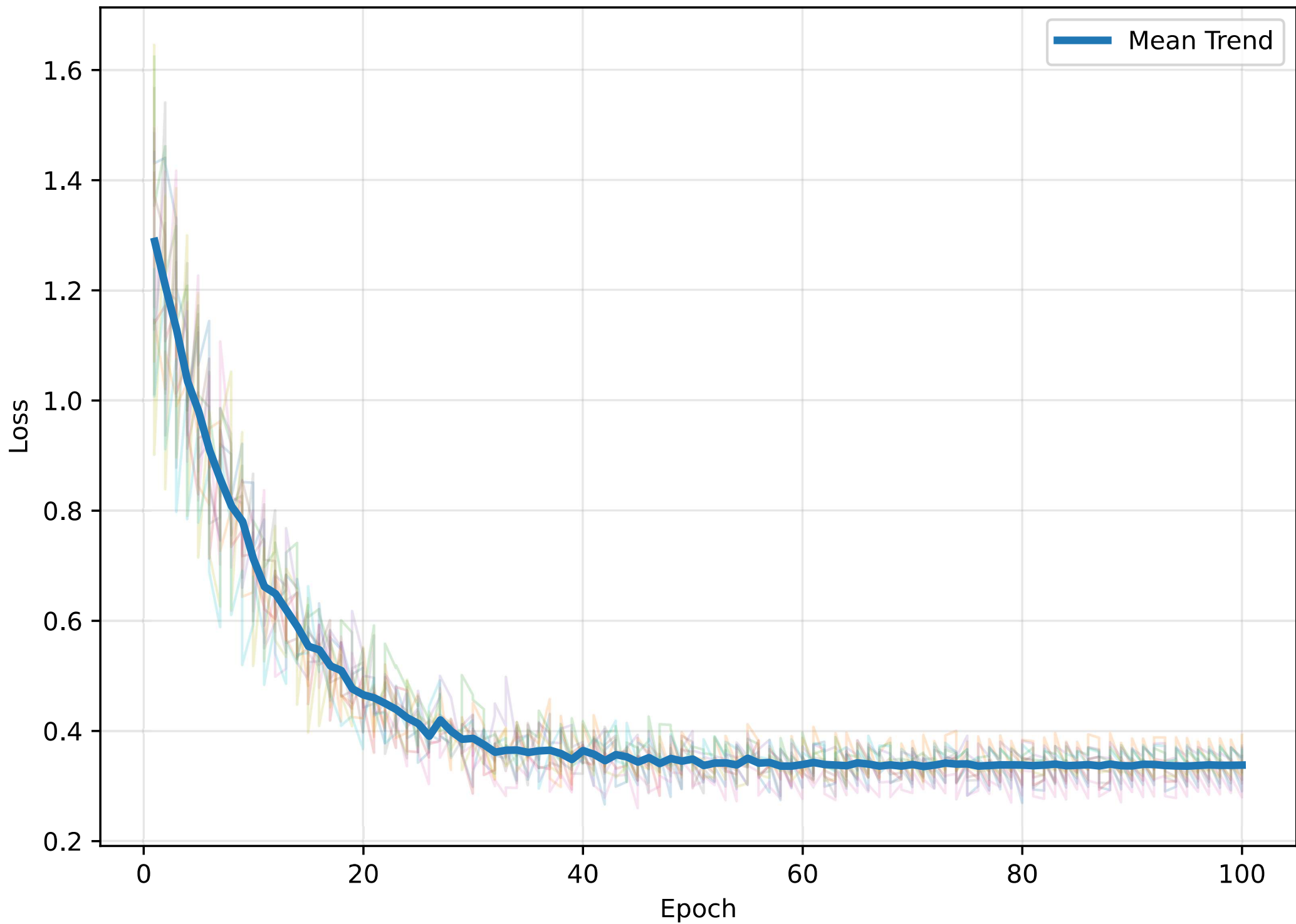
EDGE_FUSION Training Dynamics
